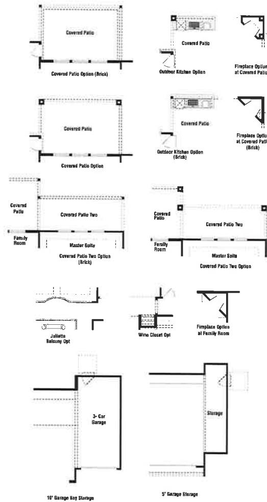
FIRST FLOOR/OPTIONS
